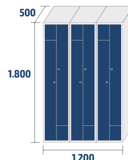
ECOL-40/3 COD: 35403 72,3kg · 1,08m 3
