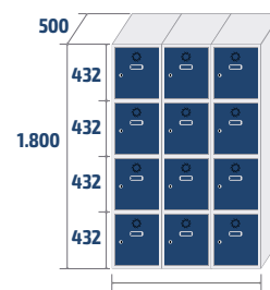
ECOC-40/3 COD: 84023 65,1kg · 1,08m 3
