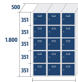
ECOP-40/3 COD: 84063 69,5kg · 1,08m 3
