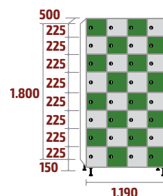
FZ-30/4 COD: 53173 201kg · 1,07m 3
