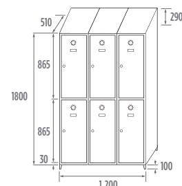
ST-40/3 INOX COD. 84913
