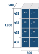
SC-40/2-PLUS
